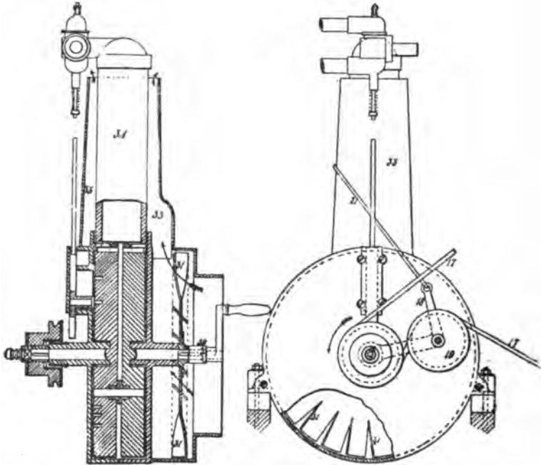
FIG. 302.—Diagram of the earliest Daimler Gasoline Motor; used on Daimler's first bicycle. The parts are indicated by numbers as follows: 17 is the driving belt passing around the pulley on the main shaft and tightened by jockey pulley, 19, and link, 21. 31 is a rotary fan, consisting of a number of radial fins as shown, which keeps a current of air passing through the air jacket, 33. 34 is the cylinder shown in part section.
